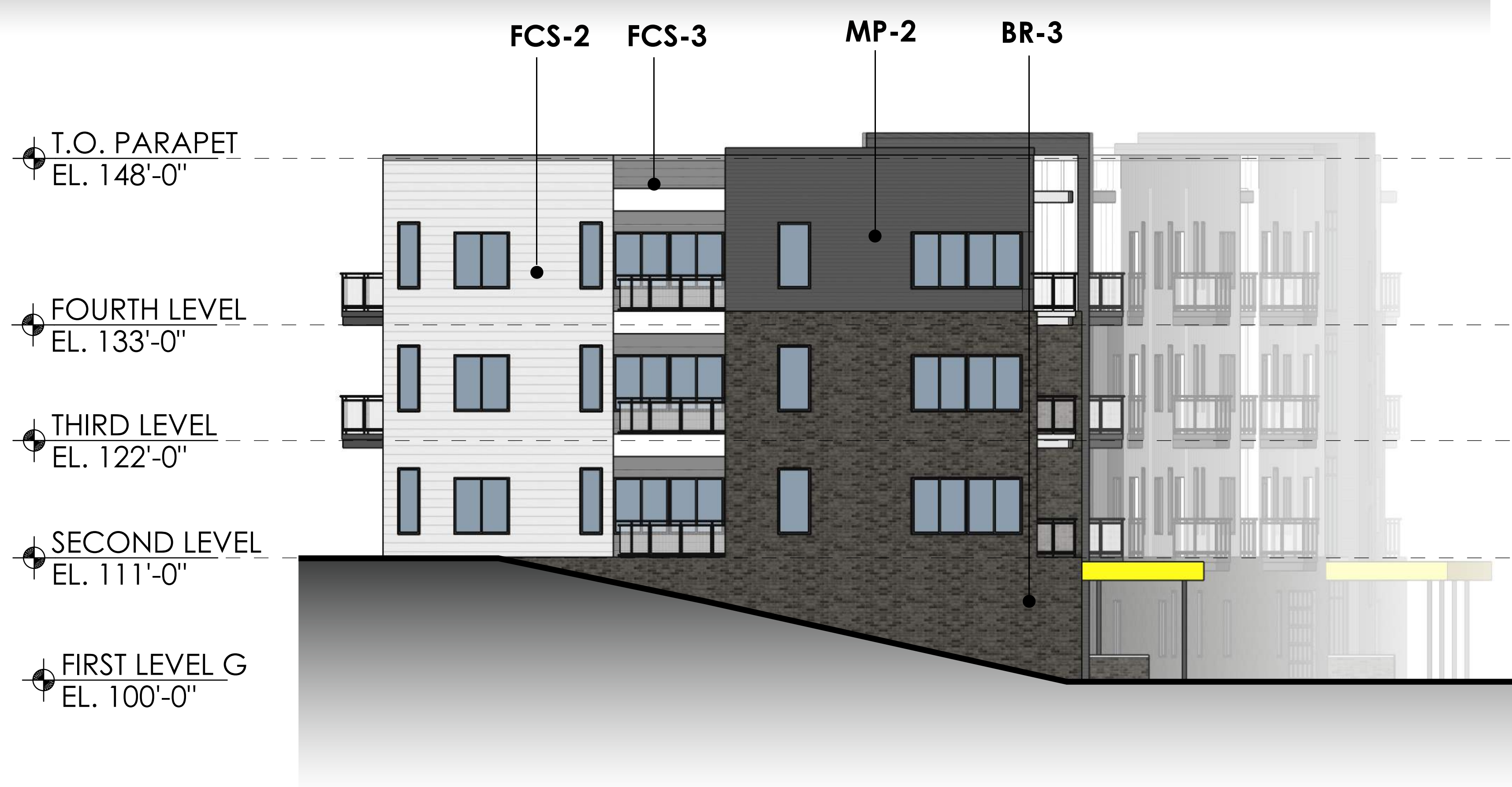
NORTH ELEVATION
