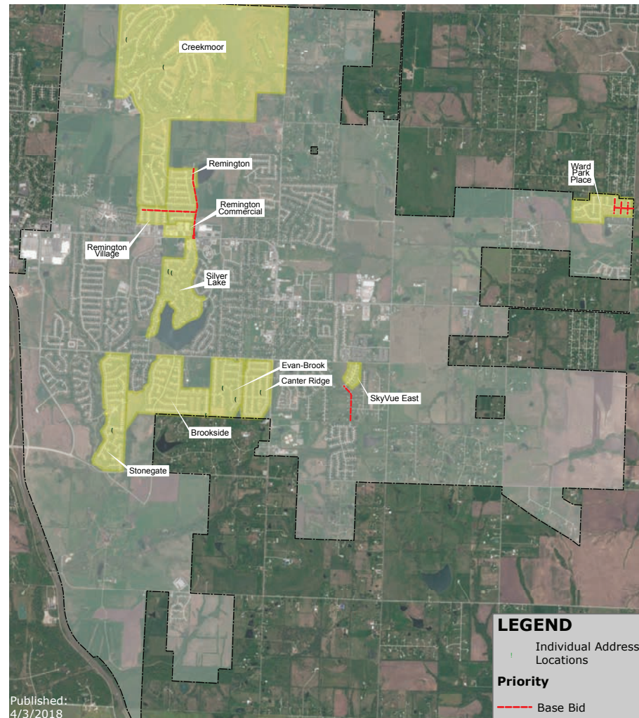
The City of Raymore's Annual Curb Replacement Plan for program year 2018.
