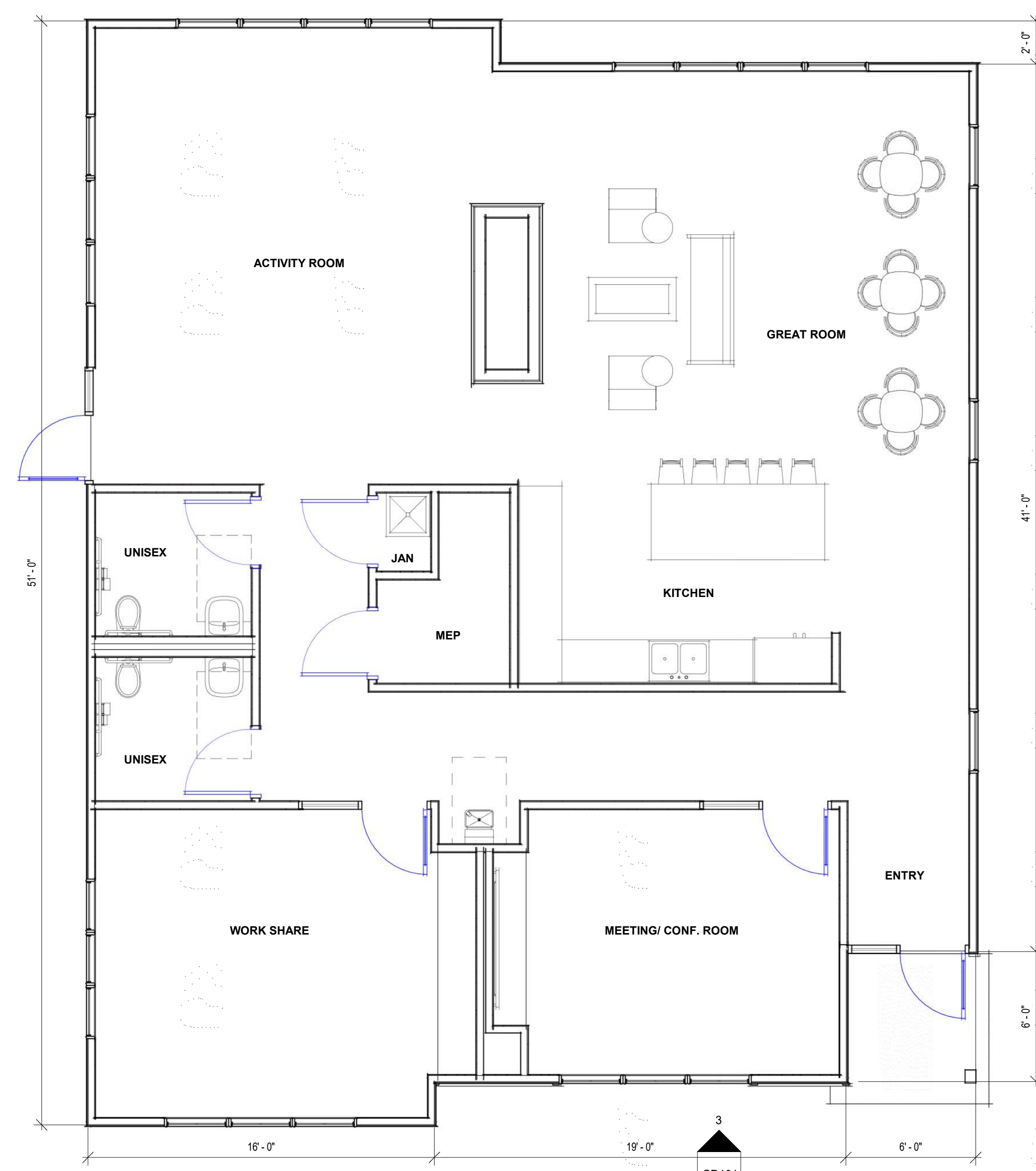
1 FIRST LEVEL - CLUBHOUSE 1/4" = 1'-0"
