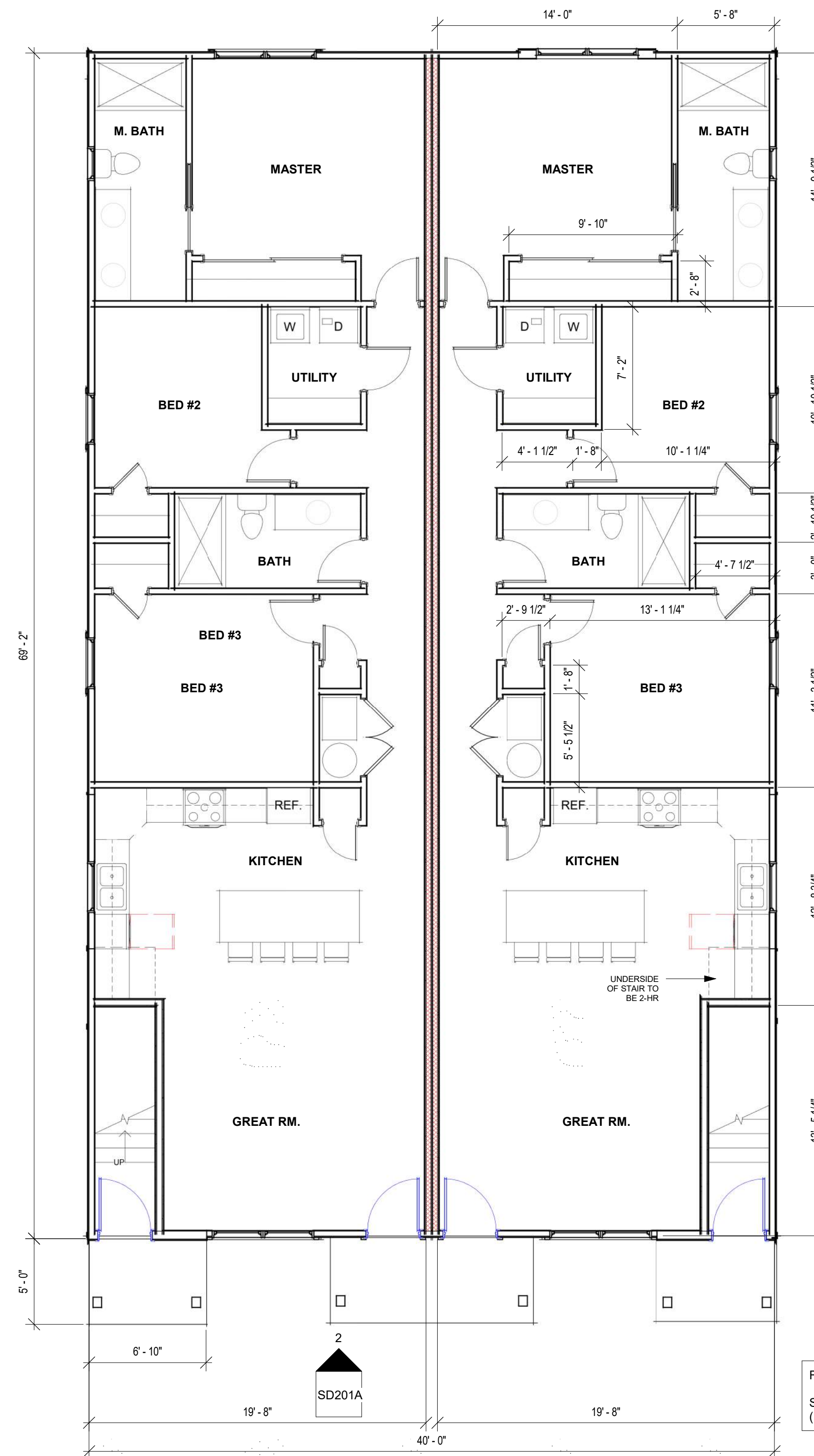
1 FIRST LEVEL - UNIT TYPE B (2 UNITS) 3/16" = 1'-0"
